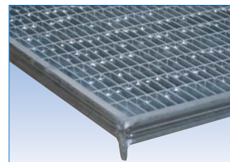
Pressed steel edge protection grilles, 30/10* mesh size for loads up to 7.2 kN
