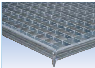
Comgrid edge protection grilles 30/30 mesh size for loads up to 6.2 kN
